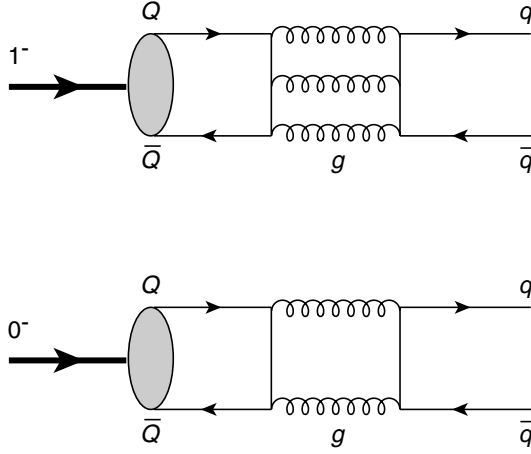
Fig. 25.1. Hadronic decays of a heavy quarkonium.
