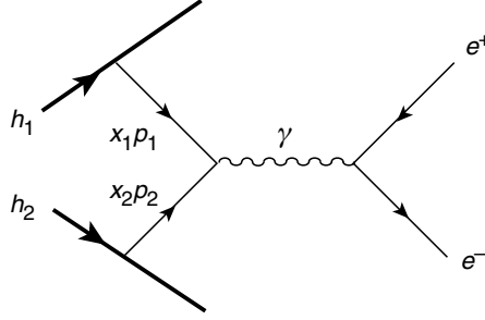
Fig. 20.1. Drell–Yan process.
