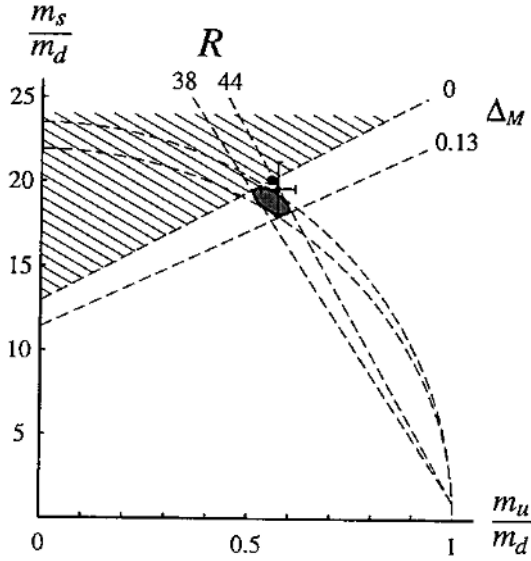
Fig. 42.1. m_s/m_d versus m_u/m_d from [57].
