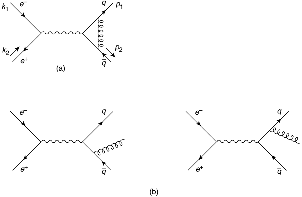
Fig. 24.1. \alpha_s corrections to e^+e^- \rightarrow \gamma^* \rightarrow \bar{q}q . (a) vertex corrections. (b) gluon radiation.
