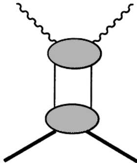
Fig. 4. The QCD-improved parton model representation.
