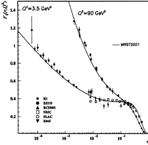
Fig. 2.7. The proton structure function F_2 versus x at two values of Q^2 , exhibiting scaling at the pivot point x \approx 0.14 .
