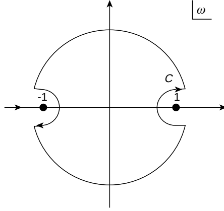
Fig. 16.1. Integration contour.
