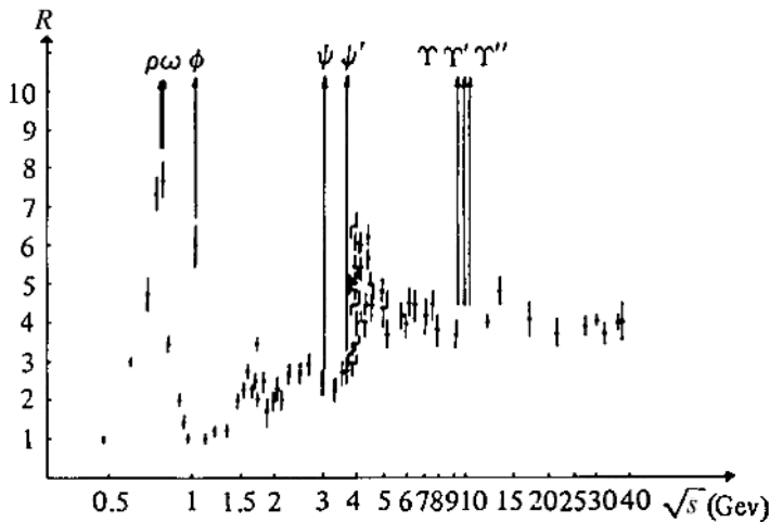
Fig. 25.2. e^+e^- \rightarrow \text{hadrons} data at lower energies.
