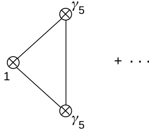
Fig. 54.4. QCD diagram contributing to the scalar \bar{q}q decay into two pseudoscalar mesons Goldstone bosons.
