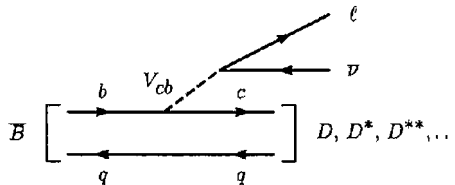
Fig. 44.4. Semi-leptonic decays of B mesons.
