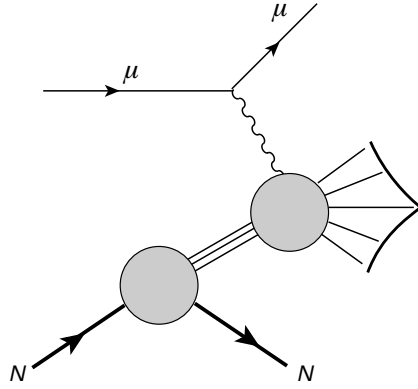
Fig. 19.2. Semi-inclusive process.
