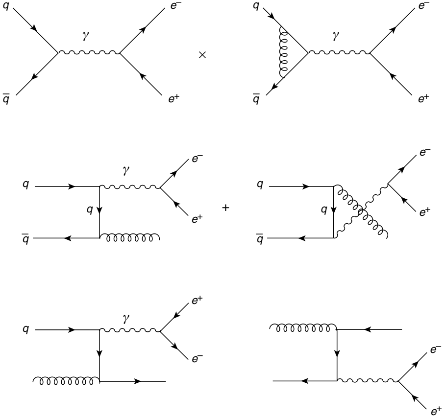
Fig. 20.2. NLO corrections to the Drell–Yan process.
