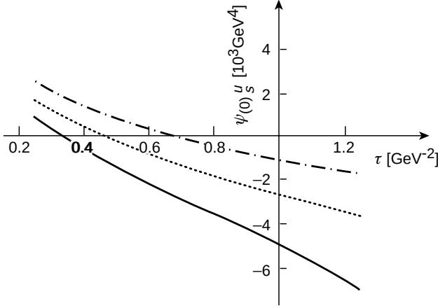
Fig. 53.8. LSR analysis of the subtraction constant \Psi(0) . We use \bar{m}_s(2) = 117.4 MeV, f_{K^*0} = 46 MeV and t_c = 6.5 GeV 2 . The curves correspond to different truncations of the PT series: to \mathcal{O}(\alpha_s) : dotted-dashed; to \mathcal{O}(\alpha_s^2) : dashed; to \mathcal{O}(\alpha_s^3) : continuous.
