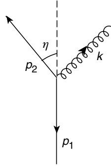
Fig. 24.4. Configuration of \bar{q}qg produced state.
