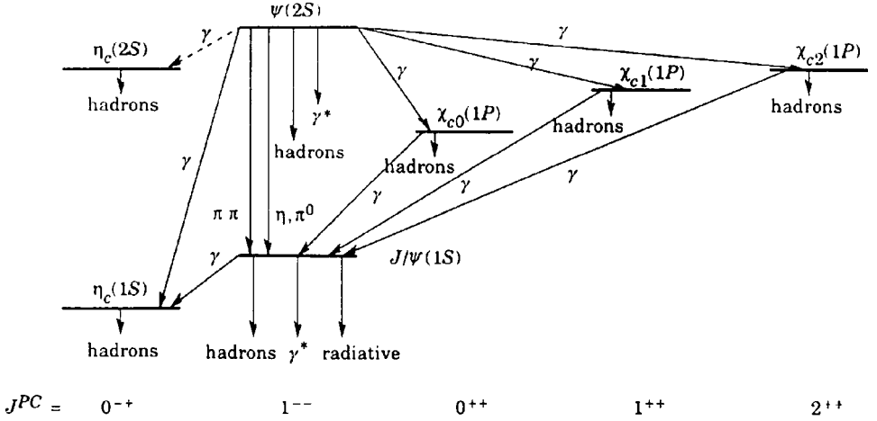
Fig. 45.1. Current situation of the charmonium system and transitions interpreted from some models. Dashed lines are uncertain states. \gamma^* refers to processes involving virtual photons, including decays into e^+e^- and \mu^+\mu^- .
