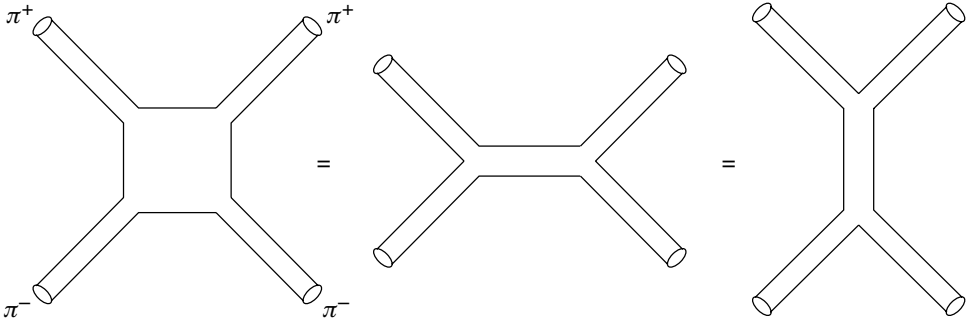
Fig. 2.10. Dual-resonance diagram for \pi\text{-}\pi scattering.
